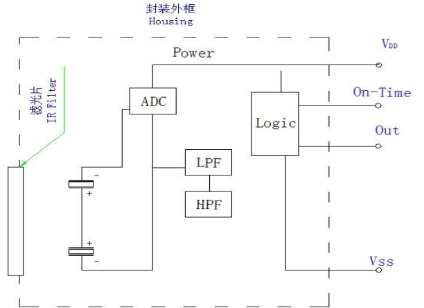
传感器等效电路图 Equivalent Circuit of Sensor
